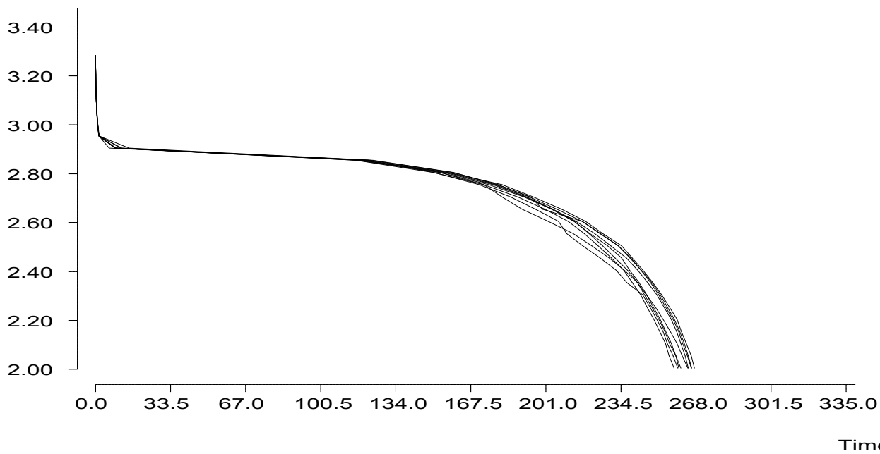
Voltage(V) Battery discharge graph
