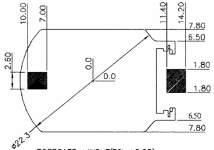
PCBBOARD LAYOUT (TOL: ±0.05)
